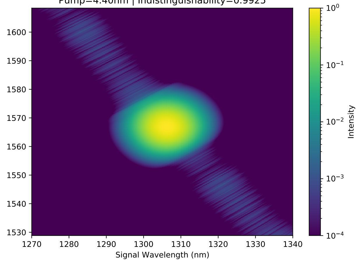
4. Optimized JSA (Exp Reconstruction, Log) Pump=4.40nm | Indistinguishability=0.9925
