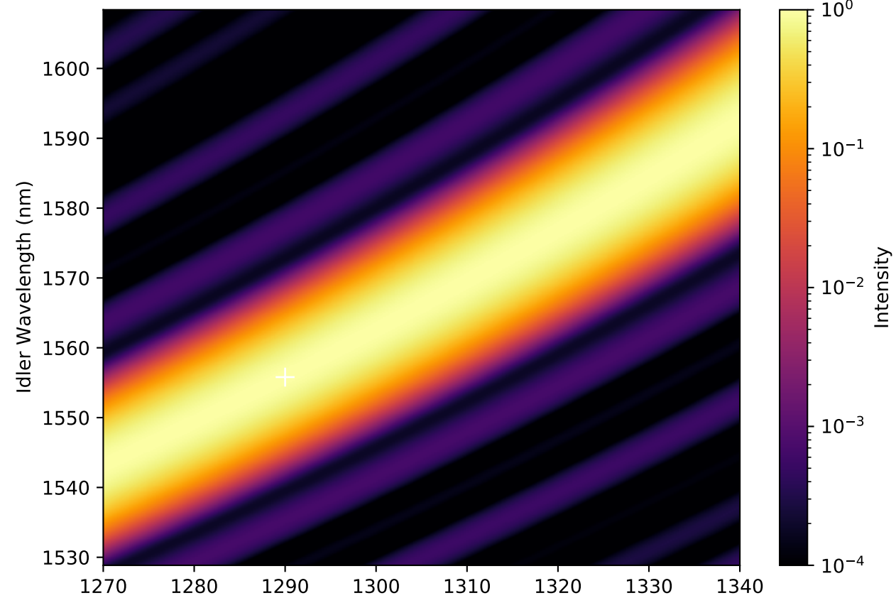
3. Optimized JSA (Theory, Log) Pump=4.40nm | Indistinguishability=0.9963
