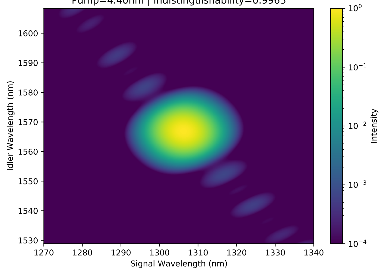
3. Optimized JSA (Theory, Log) Pump=4.40nm | Indistinguishability=0.9963
